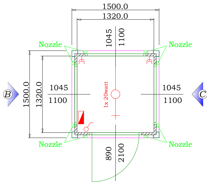
FLOORPLAN 1:40
